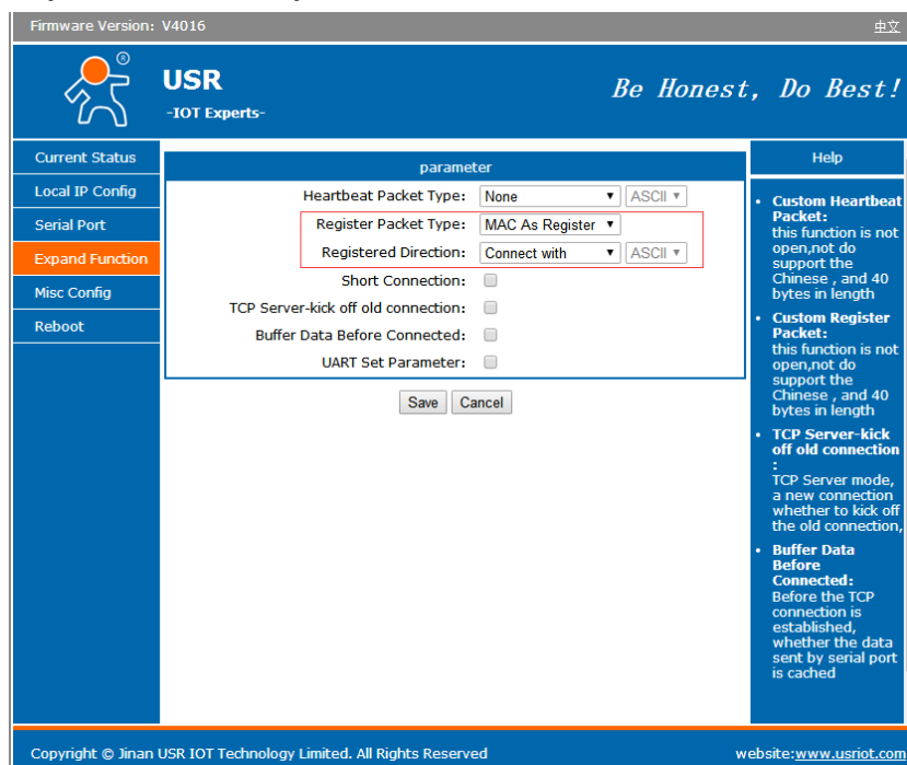
Figure 15 Identity Packet
