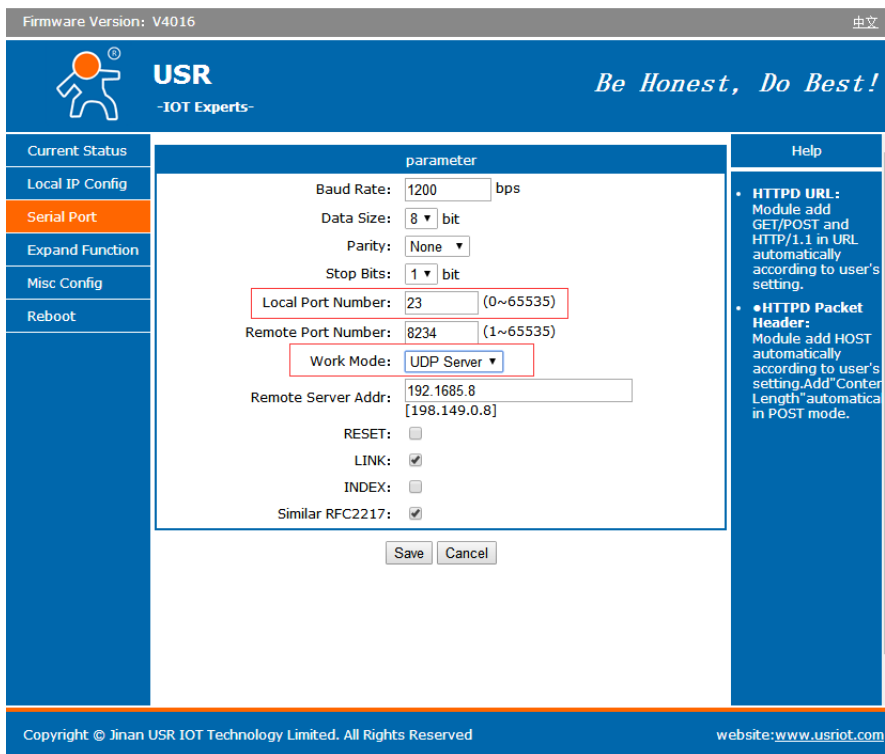
Figure 10 UDP Server
