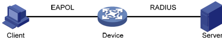
Figure 146 IEEE802.1X Structure
