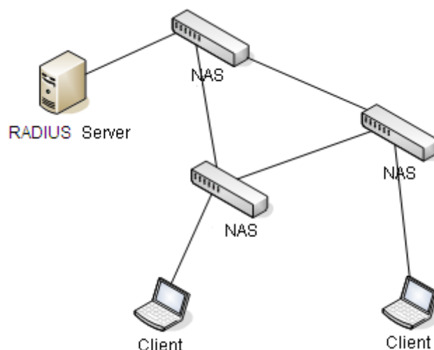
Figure 136 RADIUS Structure
