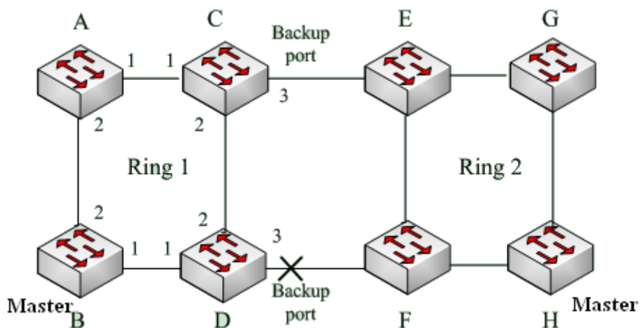
Figure 210 DT-Ring+ Topology
