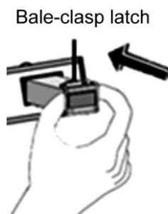
Figure 2 Installing an SFP Module
