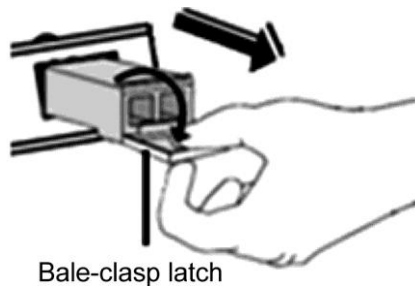
Figure 6 Removing an SFP Module 1
