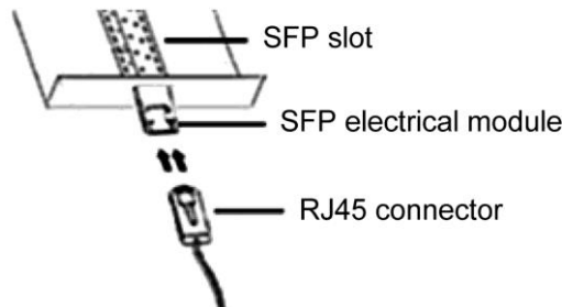
Figure 5 Connecting an SFP Electrical Module
