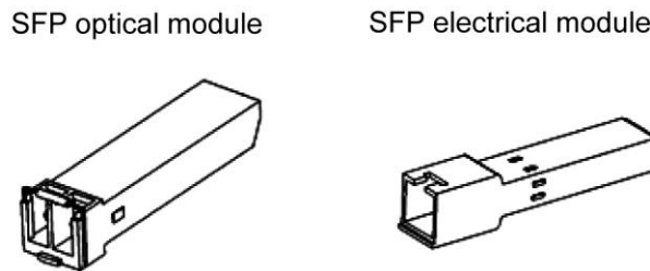
Figure 1 SFP Module
